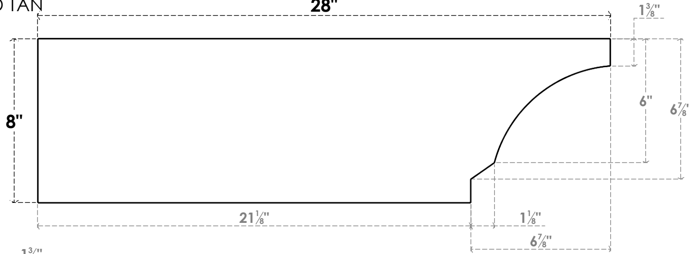
SIDE PROFILE
